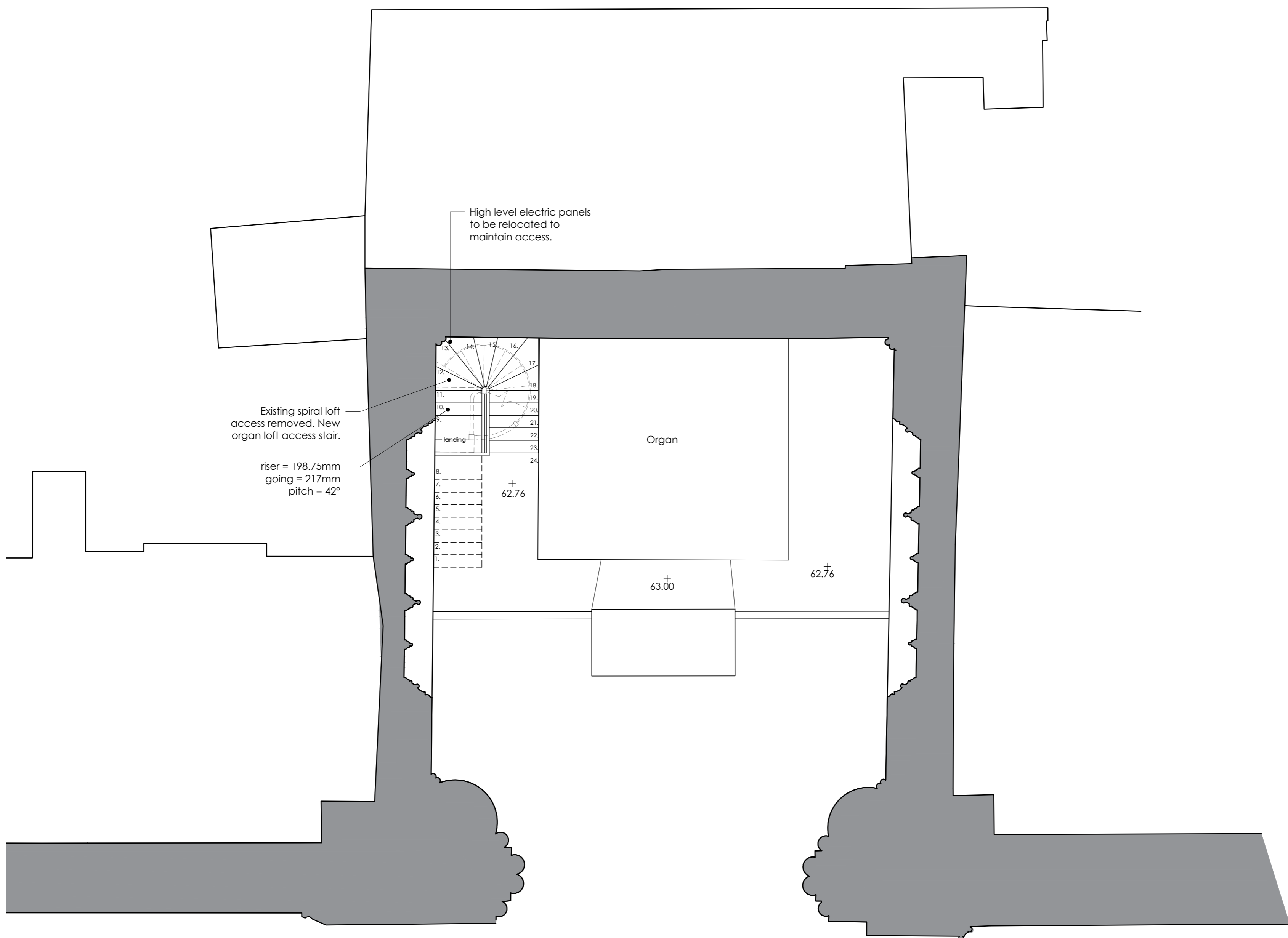
PROPOSED FIRST FLOOR PLAN
